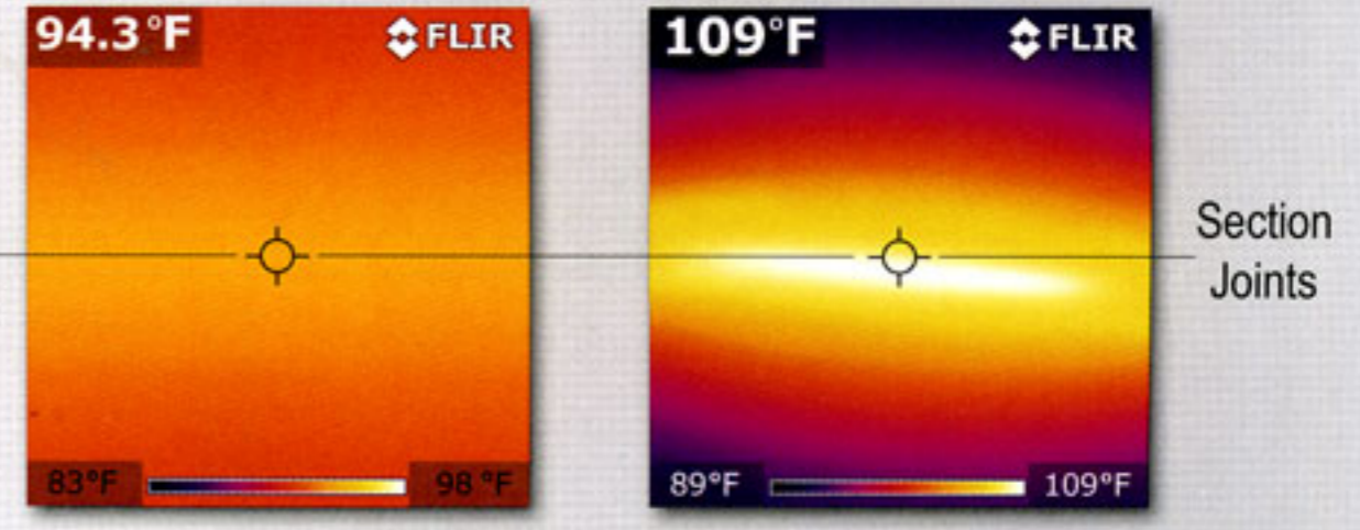
Lower Temperature with Thermal Break (Northwest Door) Higher Temperature without Thermal Break (Competitor's)
